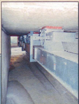
Drag Conveyor installation in a trenched commercial bin floor.
